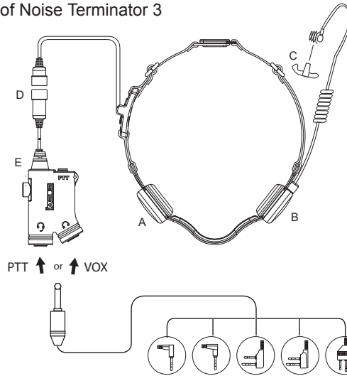
Diagram of Noise Terminator 3
